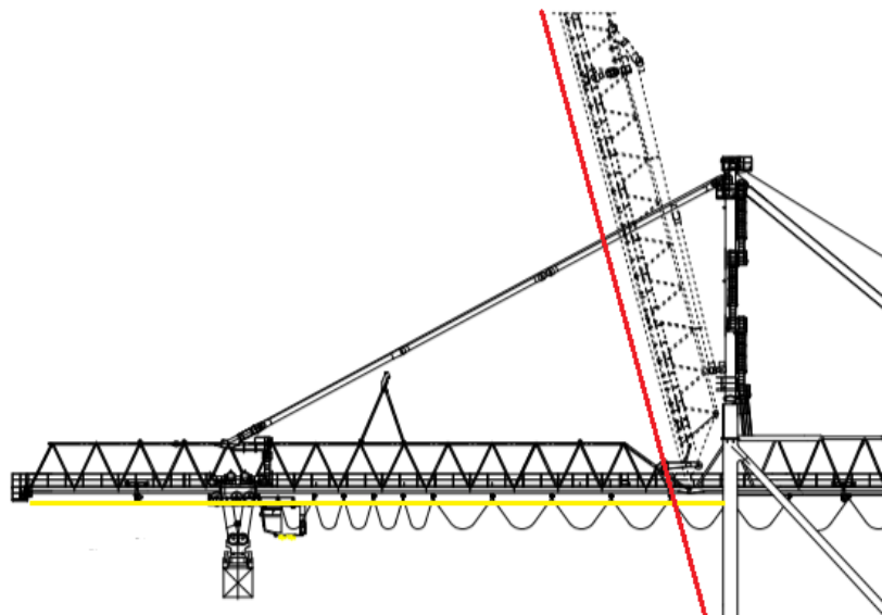
Picture 1 : Boom protecting area
